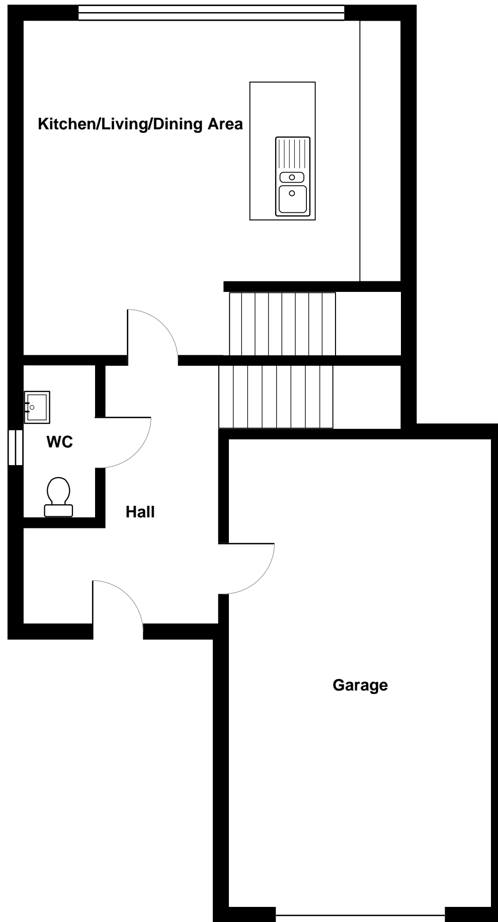
Ground Floor
